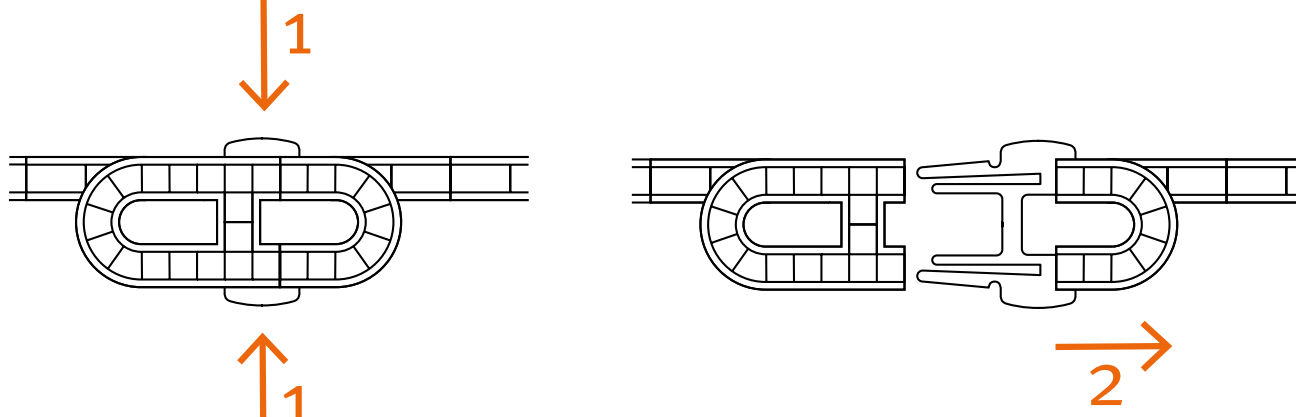
棘爪式搭扣
