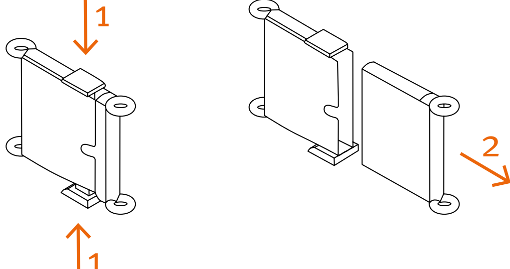
棘爪式搭扣
